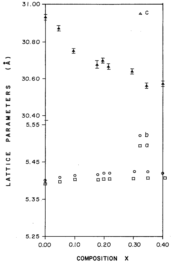
FIG. 4. Lattice parameter data for the solid solution annealed in oxygen atmosphere.
