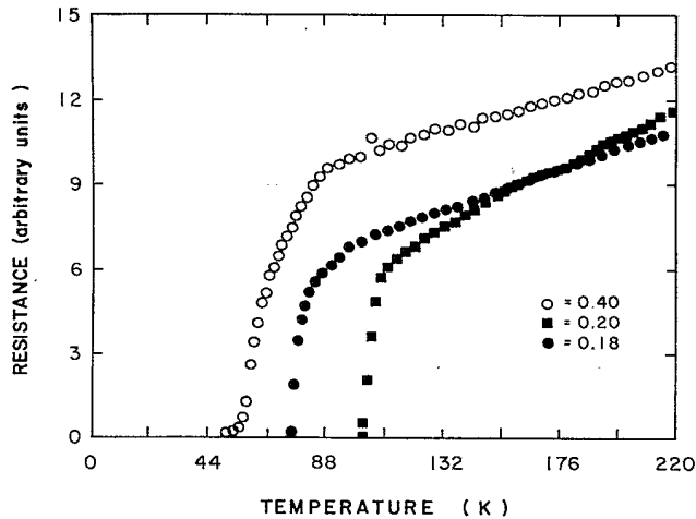
FIG. 5. A series of resistance vs temperature curves of different composition of \text{Bi}_{1.7}\text{Pb}_{0.3}\text{Sr}_{2-x}\text{Pr}_x\text{Ca}_2\text{Cu}_3\text{O}_{10+y} when x=0.18, 0.20, and 0.4 annealed in air.
