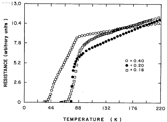
FIG. 6. Resistance vs temperature curves for samples of \text{Bi}_{1.7}\text{Pb}_{0.3}\text{Sr}_{2-x}\text{Pr}_x\text{Ca}_2\text{Cu}_3\text{O}_{10+y} with x=0.18, 0.20, and 0.4 annealed in oxygen.
